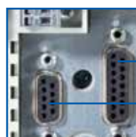
Multi encoder input Resolver input
